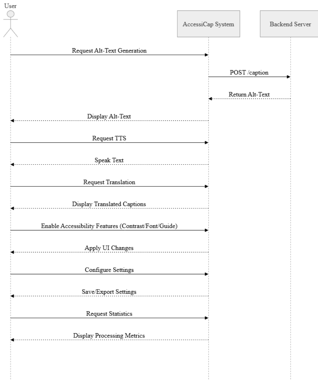
Figure 3.5: Sequence Diagram
