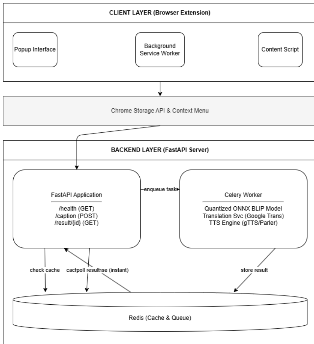
Figure 3.1: System Architecture
