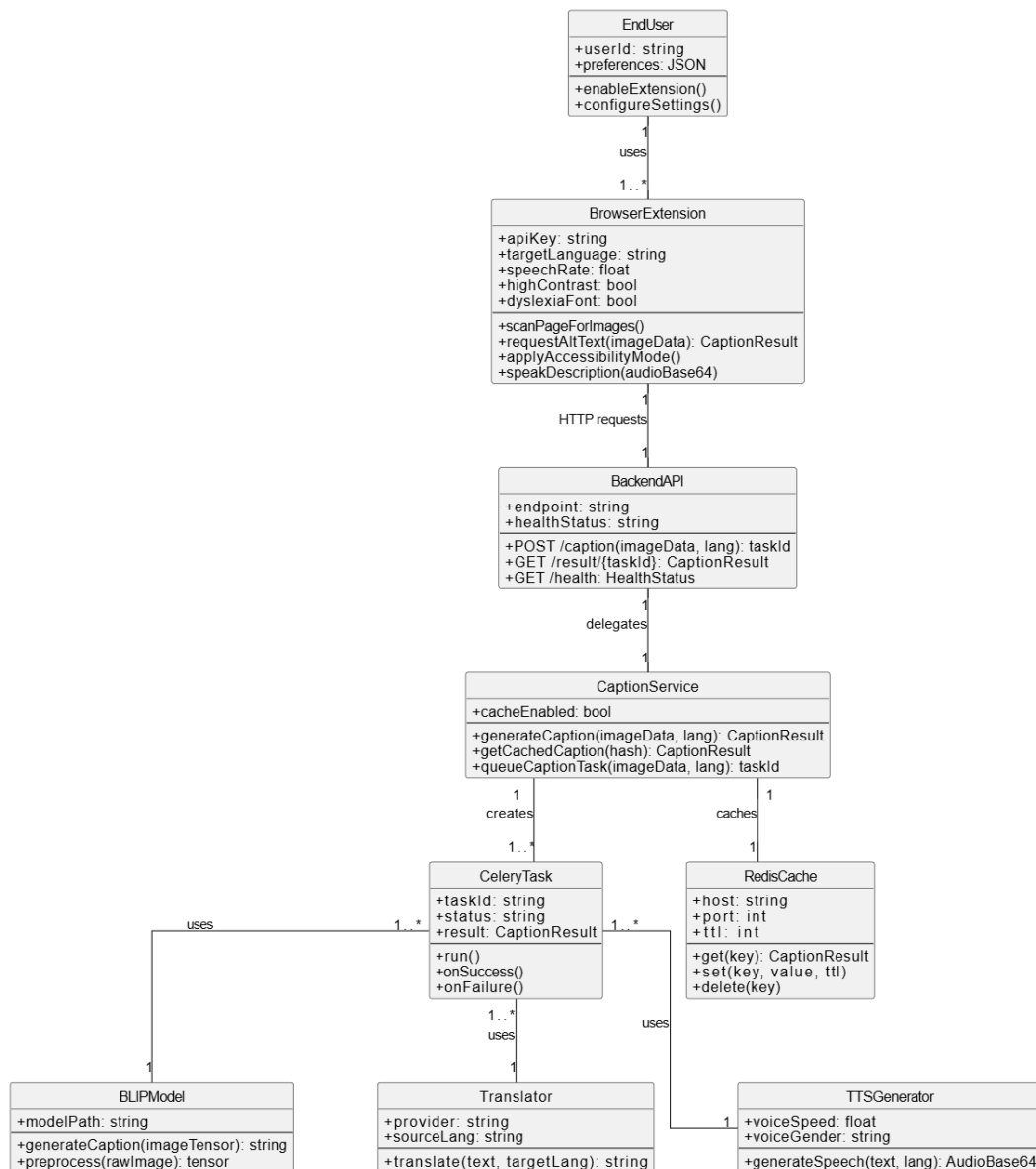
Figure 3.6: Class Diagram
